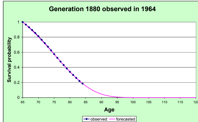
Graph 12. Observed and theoretical survival function, generation 1880, initial age 65, observation date 1964.
